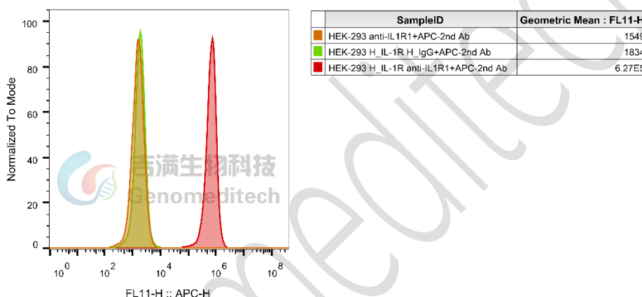
Figure 1 | H_IL-1R HEK-293 Cell Line (Cat. GM-C39967) was determined by flow cytometry using Anti-IL1R1 hIgG1 Antibody(AMG 108) (Cat. GM-51990AB ).
